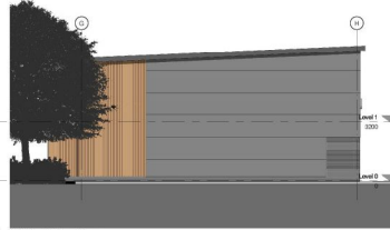
Units 6 - 8 West Elevation 1:100
